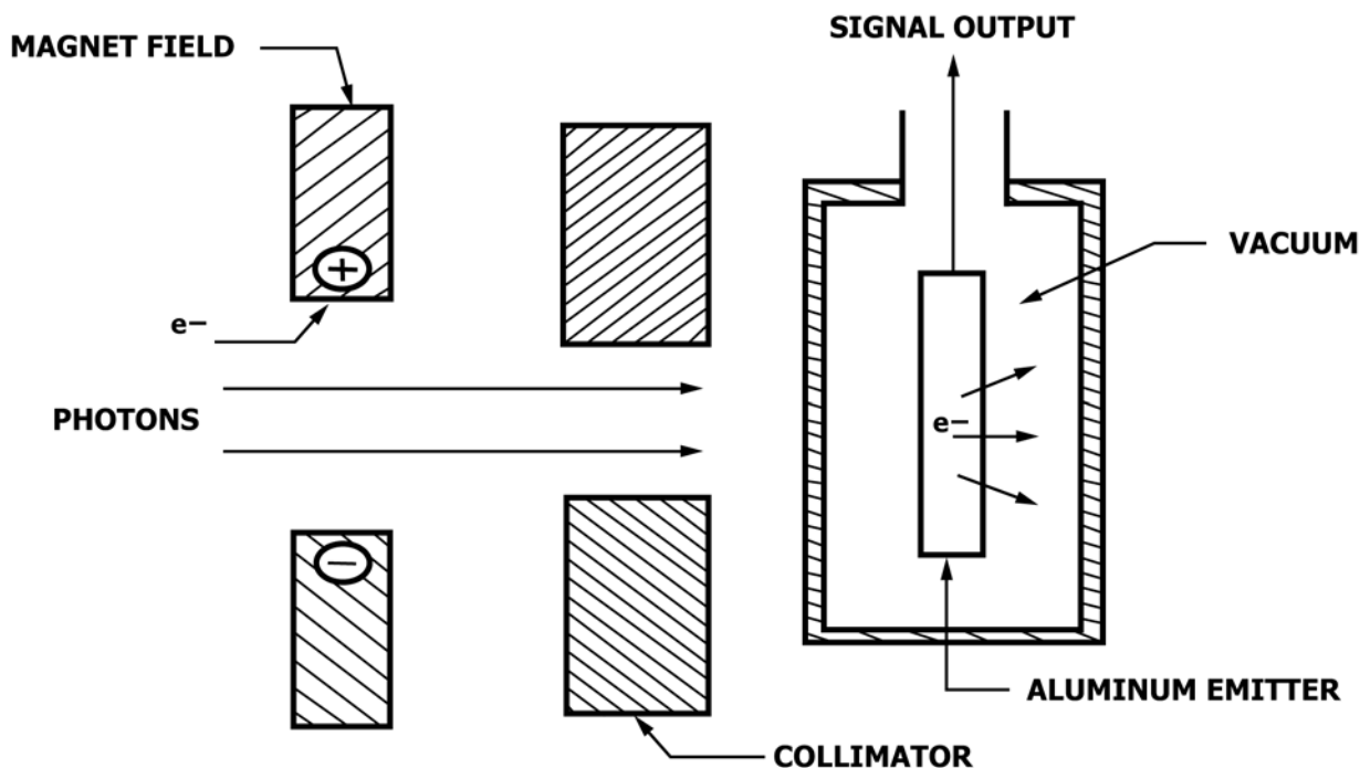
FIG. 5 Vacuum Compton Diode Schematic. Photons interact with the aluminum emitter, creating secondary electrons ( e^- ) which escape, producing an output signal (+) proportional to the rate of energy deposition.
