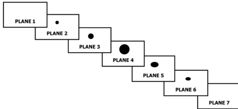
FIG. 6 Simulated CST Image Display of a Homogenous Examination Object Containing a Void
