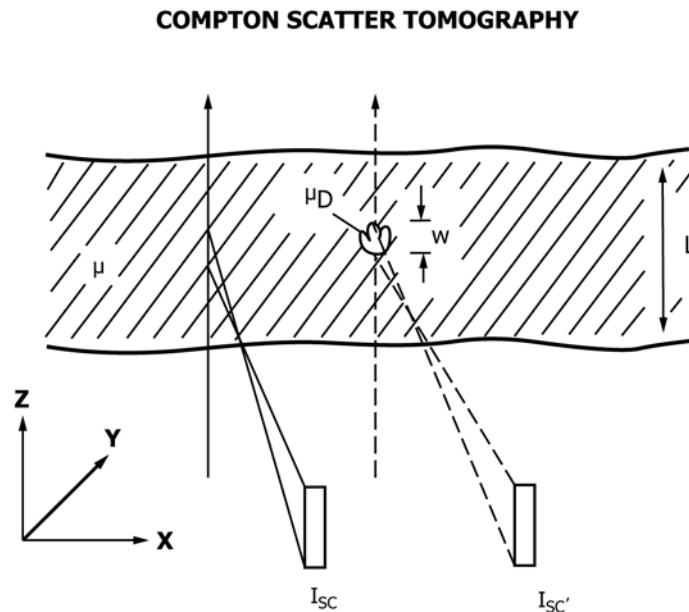
FIG. 4 Schematic Representation of the Compton Scatter Tomography Technique
