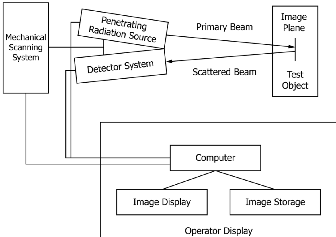
FIG. 7 Typical CST System Block Diagram
