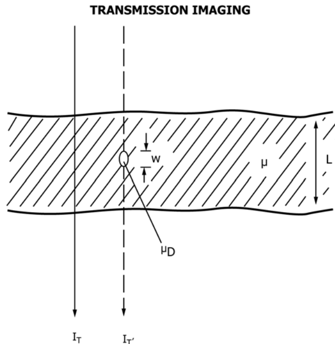
FIG. 3 Schematic Representation of the Transmitted Beam Imaging System Technique
