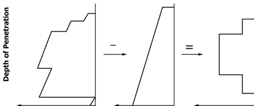
FIG. 9 CST Brightness Data Bias Caused by Differing Tomographic Plane-to-Detector Path Lengths
