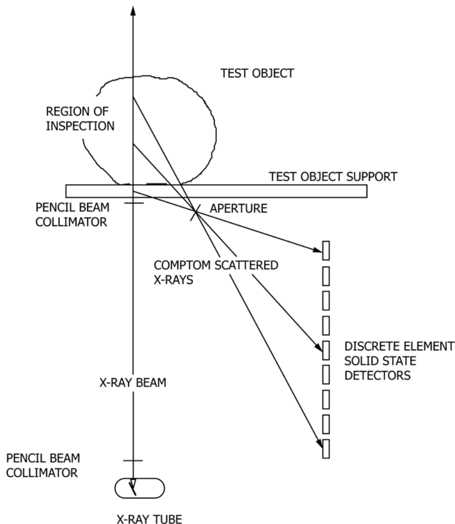
FIG. 8 General Arrangement of X-Ray Source, Detector Array and Examination Object for a Simultaneous Multi-Plane Compton Tomographic Imaging System
