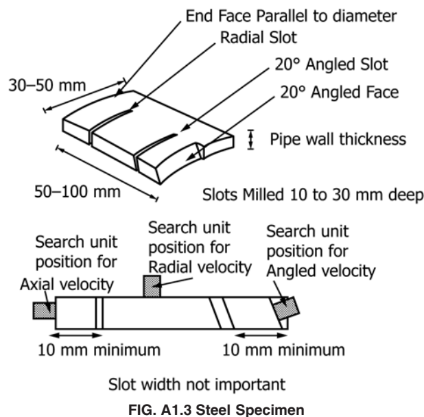
FIG. A1.3 Steel Specimen
