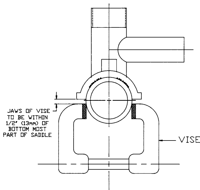
FIG. 10 Saddle Fitting Crush Test Before Crush
