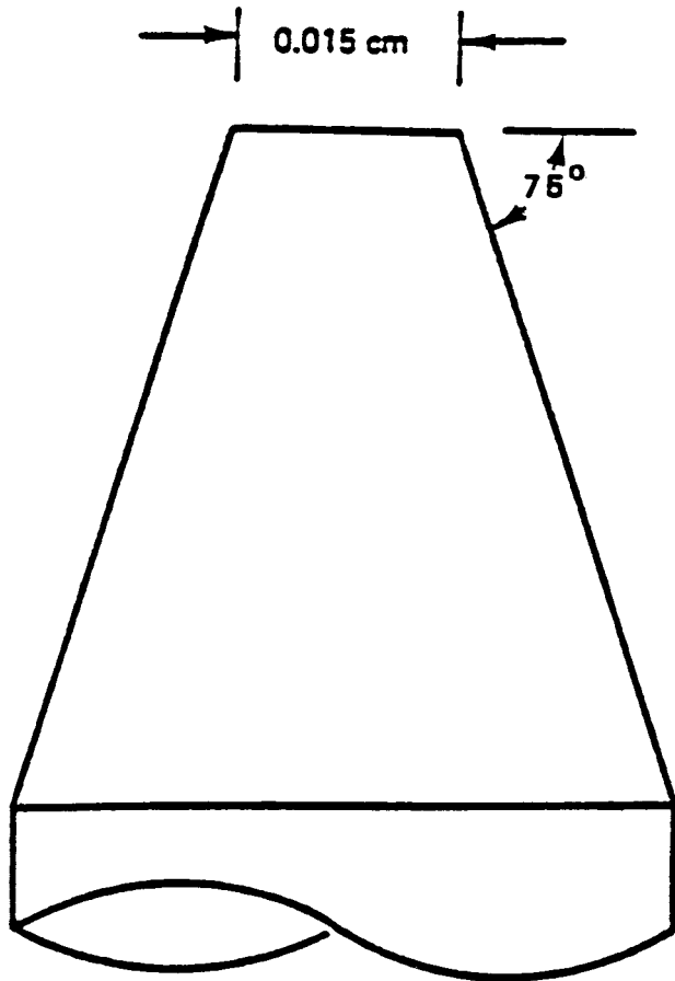
FIG. 5 Schematic Representation of Shearing Tool 25.4-μm Diameter Wire
