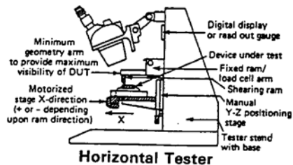
FIG. 7 Shear Tester Configurations
