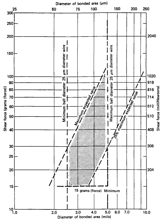
FIG. 8 Ball Bond Shear Strength Window—25.4- \mu\text{m} -Diameter Gold Wire Bonded to Aluminum Pad Metallization (The data may be extrapolated for fine pitch ball bonds. The shear force values may not be valid for copper ball bonds)
