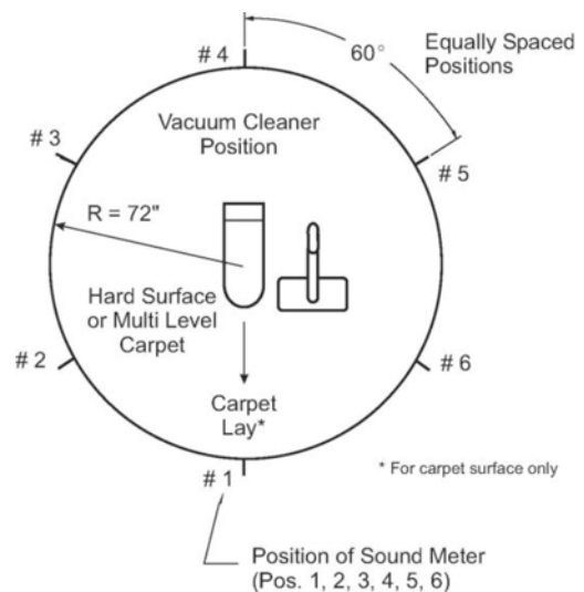
FIG. 3 Sound Test Pattern for Canisters
