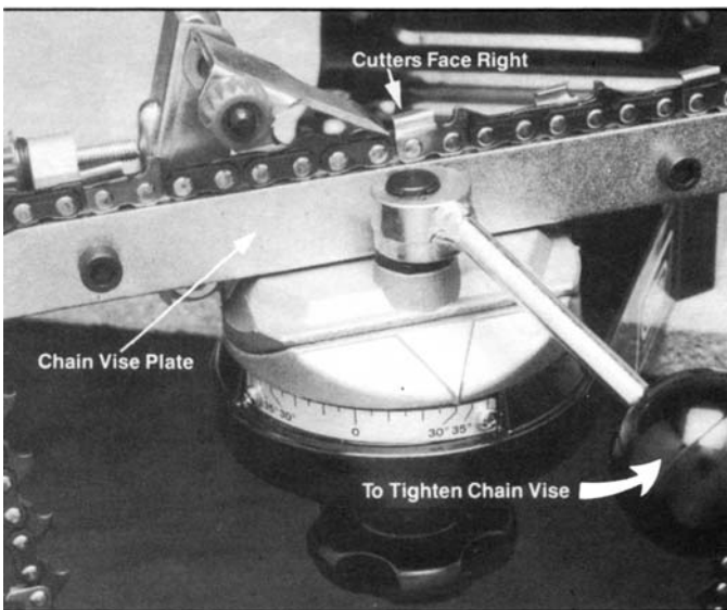
FIG. A1.8 Chain Vise Locking Knob
