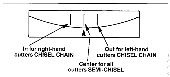
FIG. A1.4 Angle Jig
