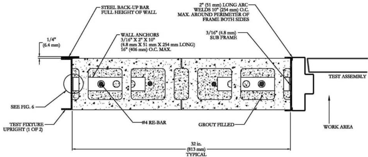
FIG. 5 Section B-B from Fig. 4
