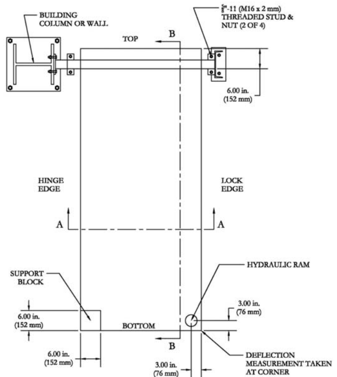
FIG. 10 Rack Test Fixture (Plan View)
