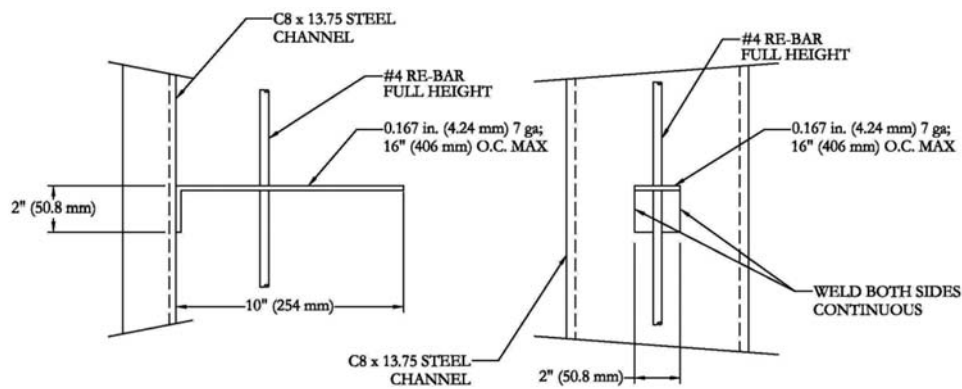
FIG. 7 Wall Anchor Welding Detention Hollow Metal Vision Systems
