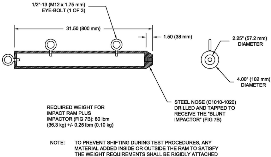
FIG 7A: STEEL IMPACT RAM
