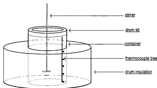
FIG. 1 Water-Bath Calorimeter
