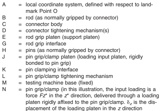
FIG. A2.1 Schematic for Testing an External Fixator Connector (Example, Generic for a Pin-Rod Joint)
