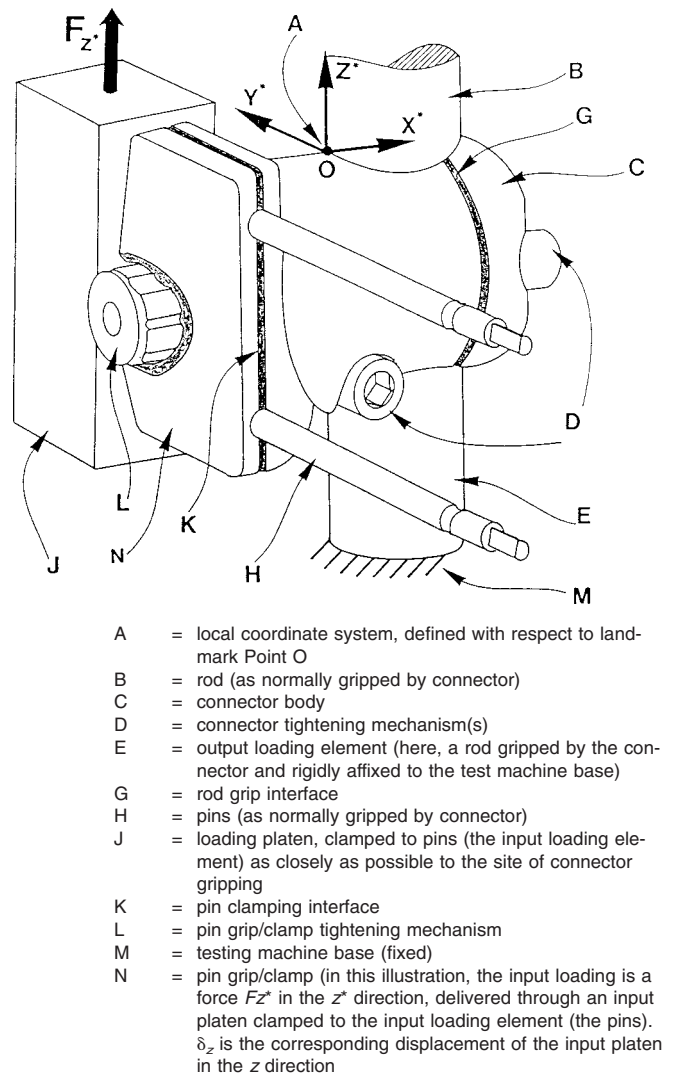
FIG. A4.1 Schematic for Testing an External Fixator Joint (Example, Generic for a Pin-Rod Joint)
