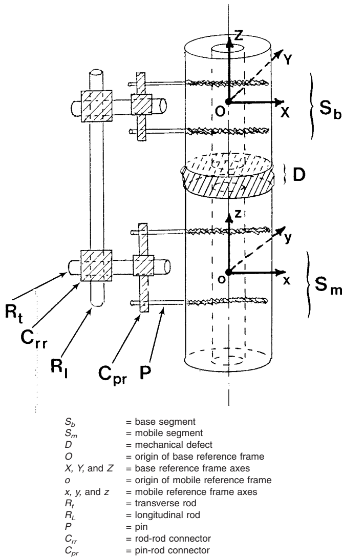
FIG. A1.1 External Fixator Definition Schematic
