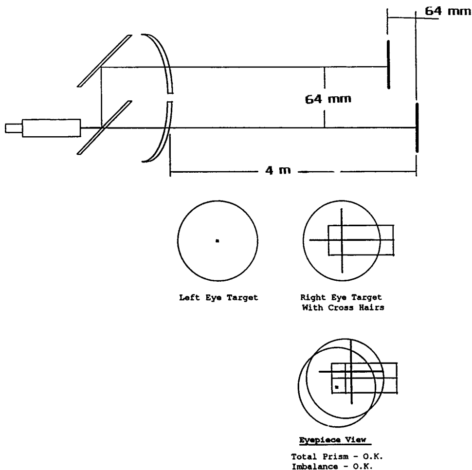
FIG. 5 Alternate Prism Test Set-Up (See 6.8.1)
