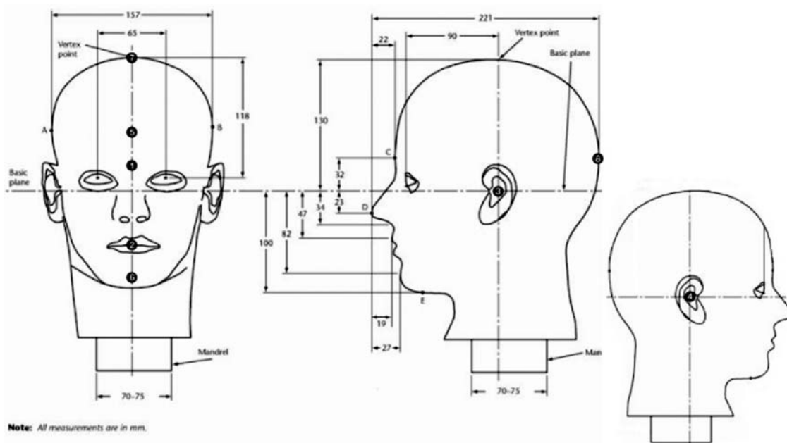
FIG. 6 Headform Details to Determine Coverage Level of EHPD
