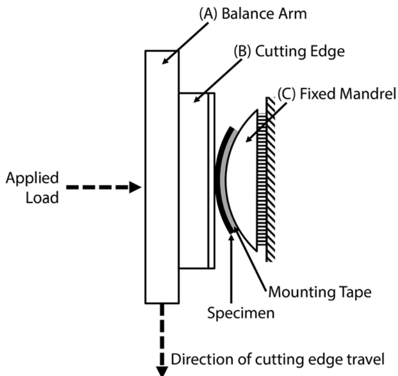
FIG. 1 Schematic of Cut Test Principle
