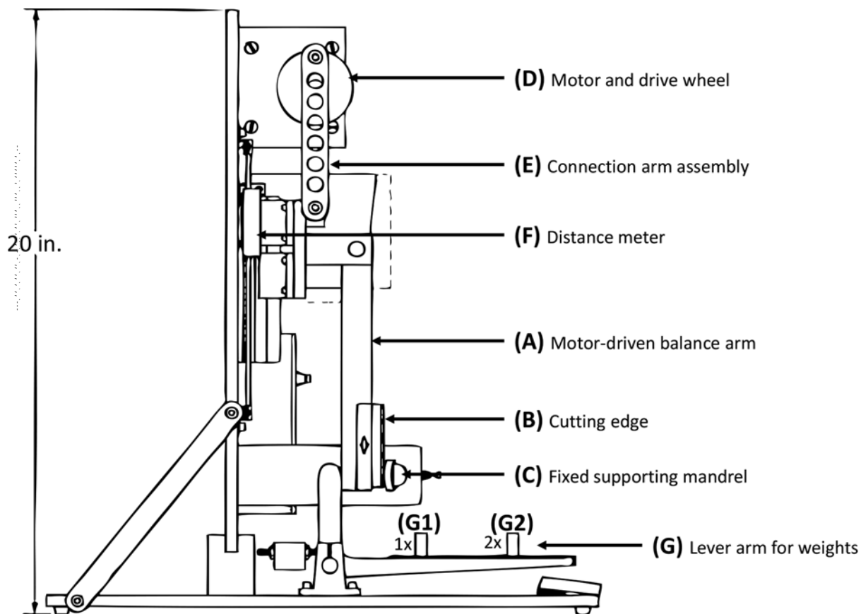
FIG. 2 Schematic of the CPP Tester (Side View)
