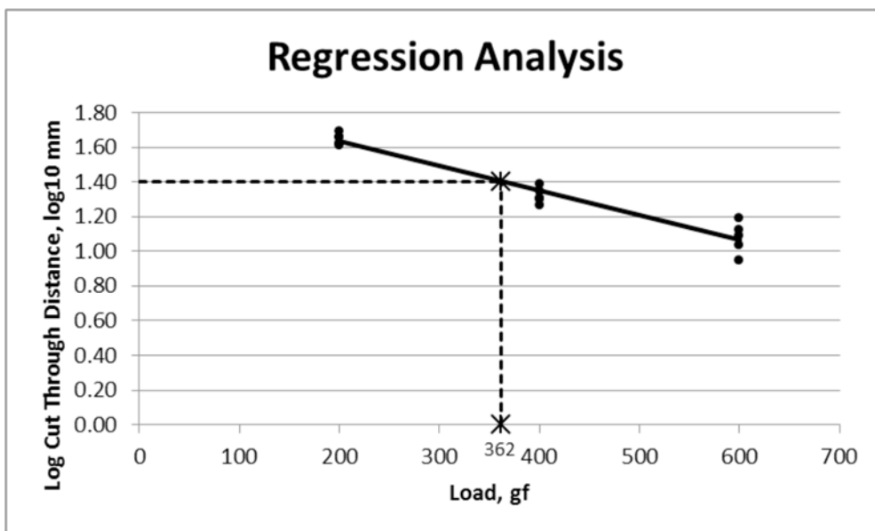
FIG. A1.1 Plot of Applied Load Versus the Log of Normalized Cut Through Distance and Resulting Regression Line and Rating Load
