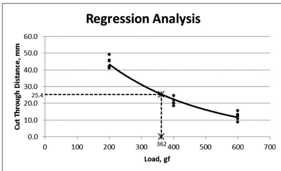
FIG. A1.2 Plot of Applied Load Versus the Normalized Cut Through Distance and Resulting Regression Line and Rating Load
