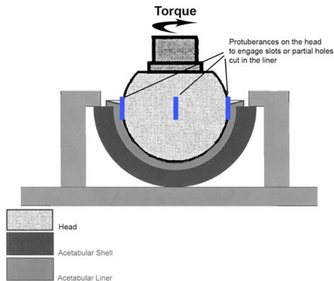
FIG. 4 Schematic of Torque Out Disassembly
