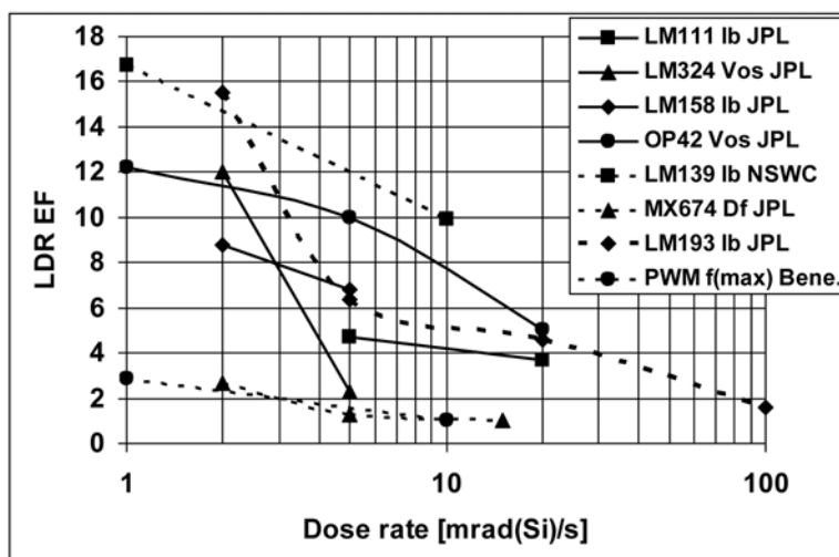
FIG. X2.10 Low Dose Rate (LDR) Enhancement Factor (EF) versus Dose Rate for Several Circuits (Ref 89)
