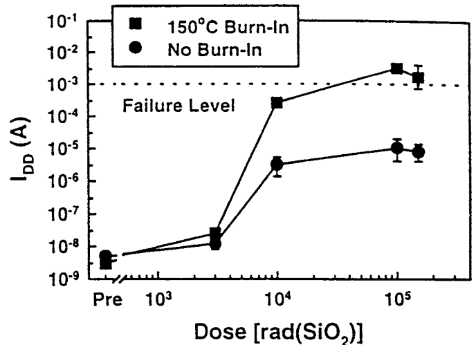
NOTE 1—The dashed line represents a parametric failure level of 1 mA. (Ref 28)
