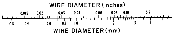
FIG. 5 Nomograph of Pull Test Loads for Various Wire Diameters and Seal Areas
