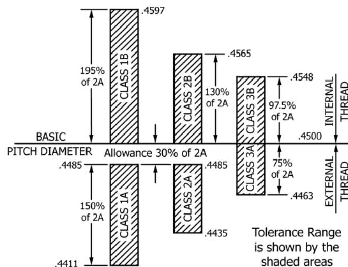
FIG. X3.1 Relationship of Pitch Diameter Allowance for Classes of Fit on \frac{1}{2} -13 UNC Thread
