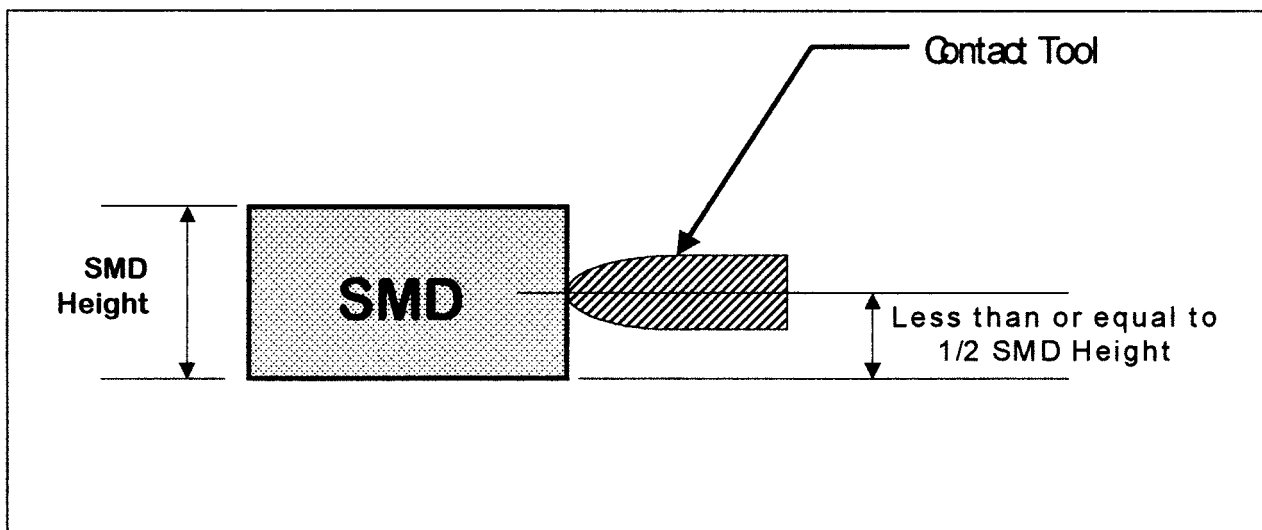
FIG. 1 SMD Contact
