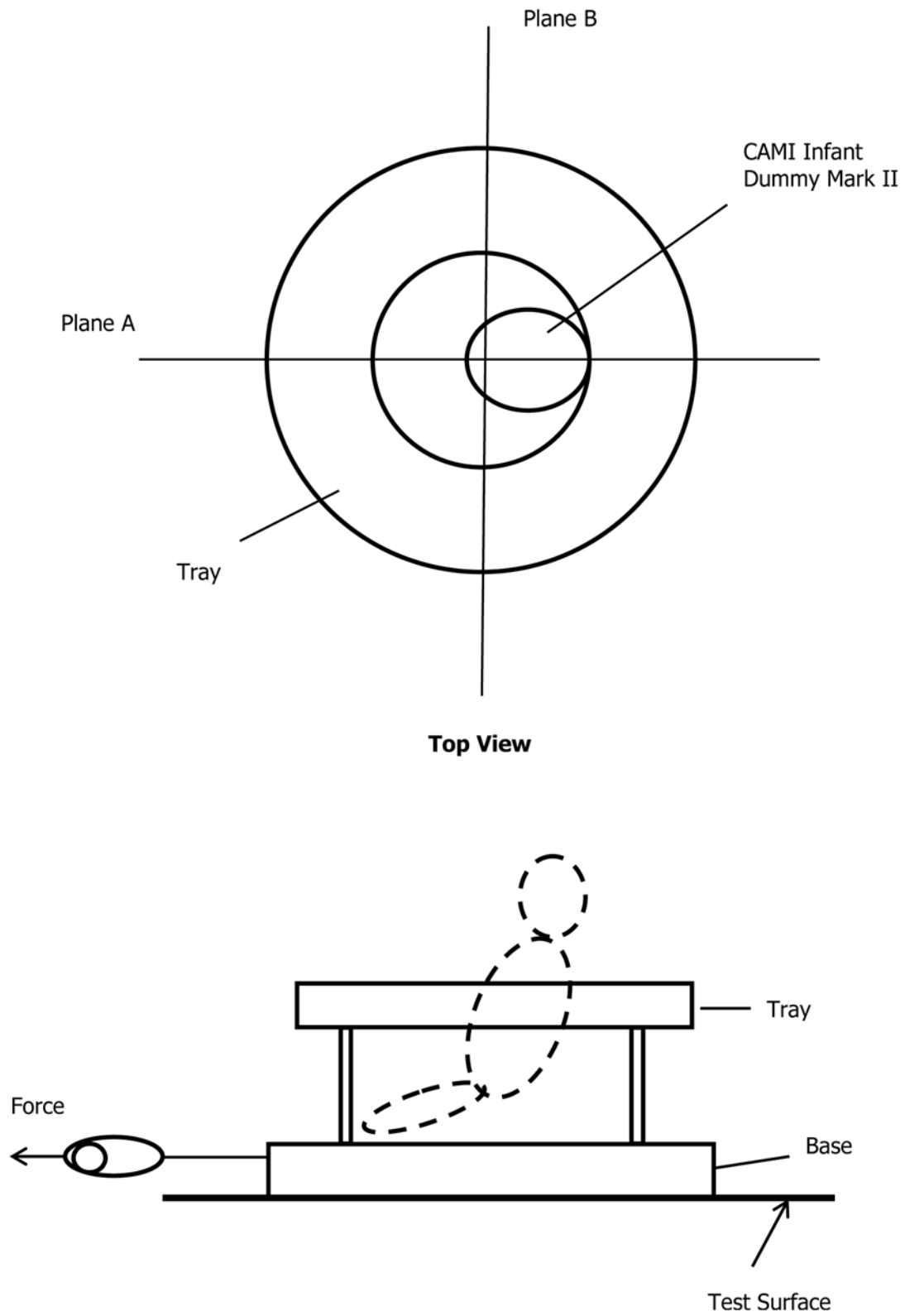
FIG. 7 Resistance to Motion Test (Ref: 7.6.1)
