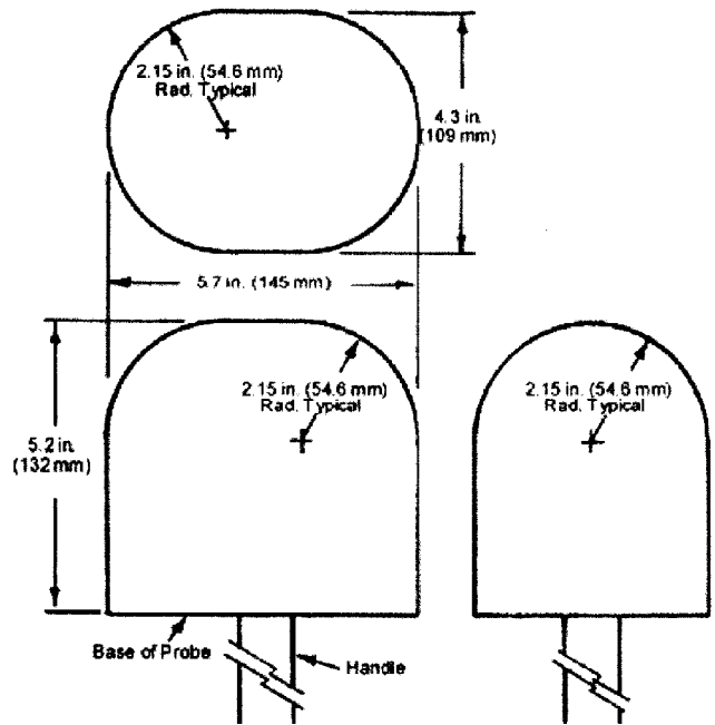
FIG. 3 Small Head Test Probe
