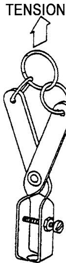
FIG. 6 Tension Test Adaptor/Clamp
