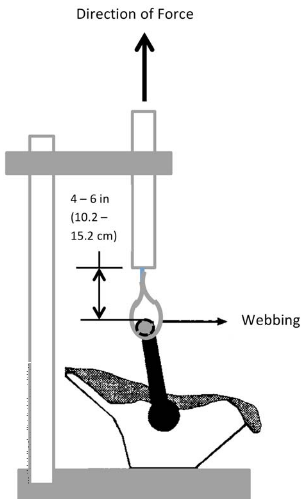
Handle Auto-lock Test
