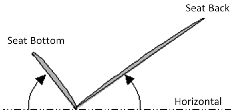
FIG. 12 Angles From Horizontal to Seat Bottom and Back
