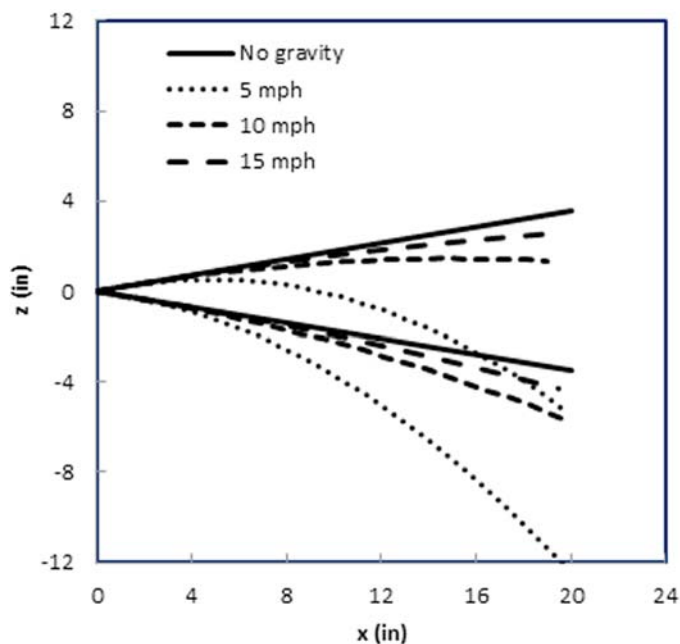
NOTE 1—Bat-ball impact is at x = 0 . Lines for each speed represent limit trajectories for softball impact rebound angles of \pm 10^\circ .
