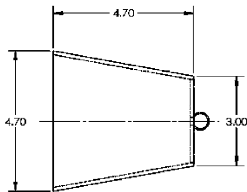
FIG. 1 Truncated Test Cone
