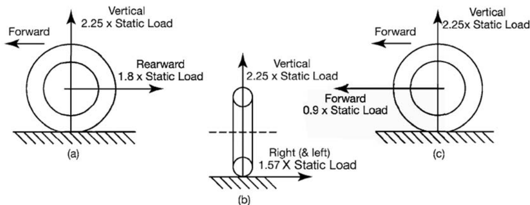
FIG. 5 Supplementary Conditions for Tail Wheel
