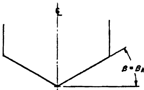
Unflored Bottom
