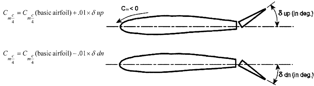
FIG. X2.2 Unsymmetrical Wing Loads
