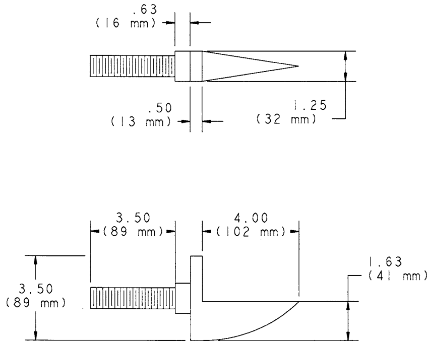
FIG. 7 Sharp Impactor
