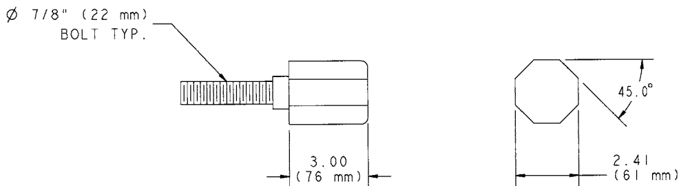
FIG. 6 Large Blunt Impactor
