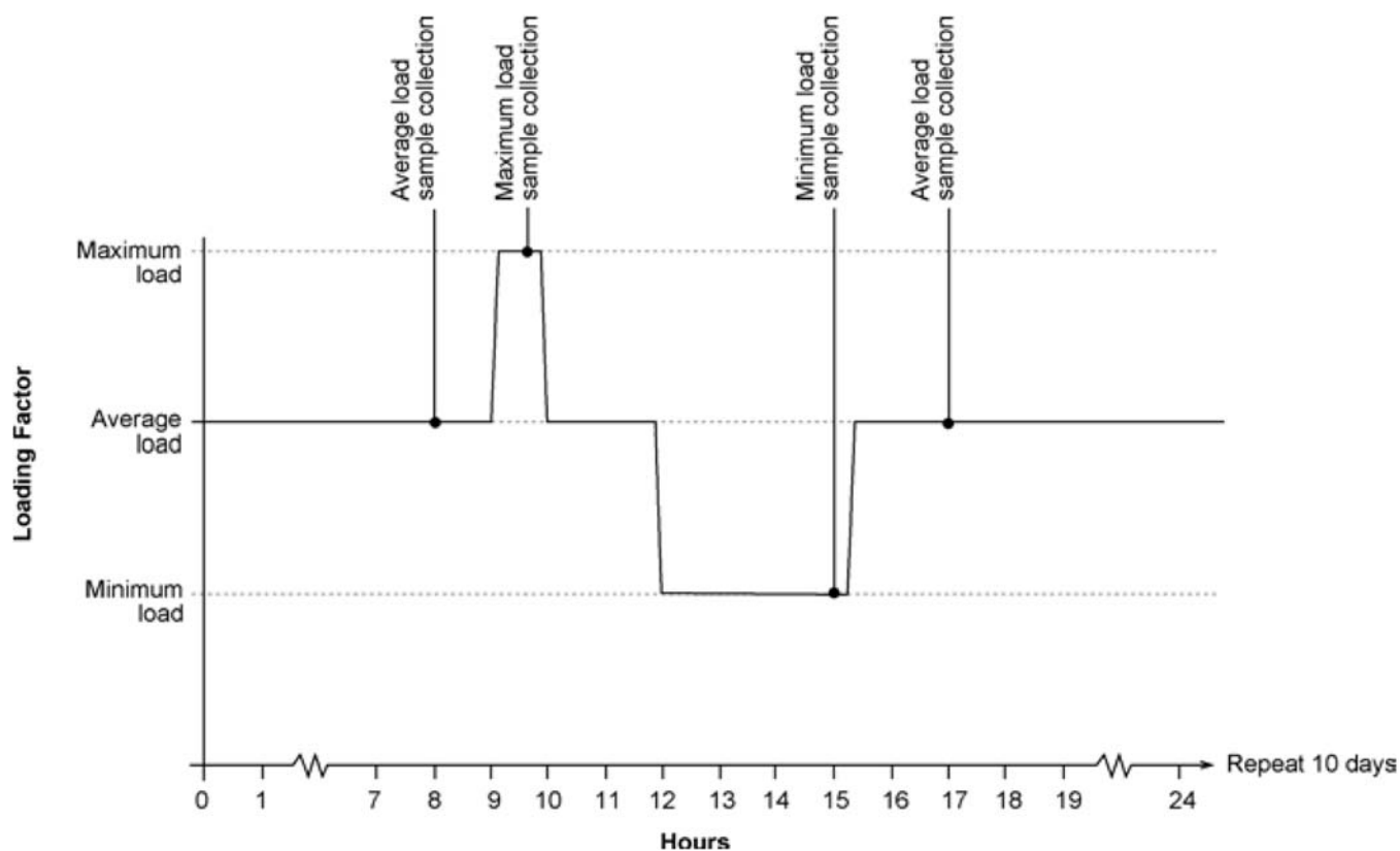
FIG. 1 Sampling Frequency for Testing Treatment Systems
