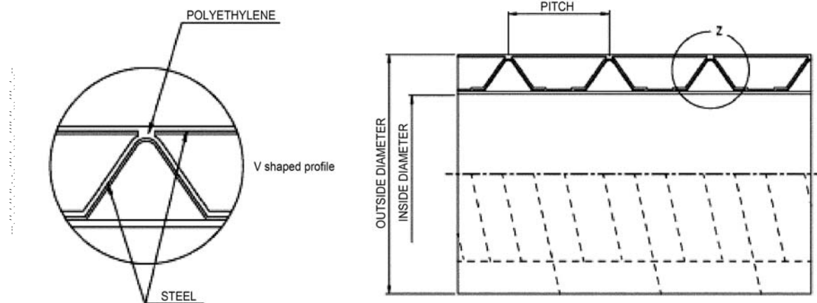
FIG. 3 Triple-Wall Steel Reinforced Corrugated Polyethylene Pipe – Type IIA
