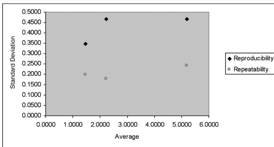
FIG. 4 Standard Deviations of Reproducibility and Repeatability Versus Average
