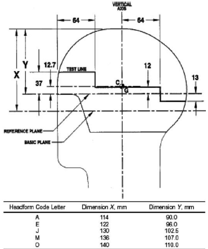
FIG. 2 Headform Basic Data and Test Line
