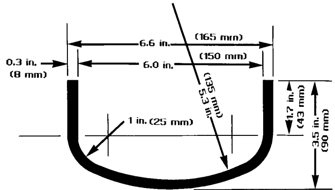
FIG. 6 Standard 6 in. (150 mm) Weld Cap
