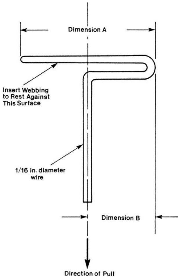
FIG. 3 Webbing Tension Pull Device
