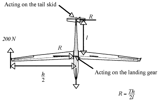
FIG. 3 Wing-Tip Landing
