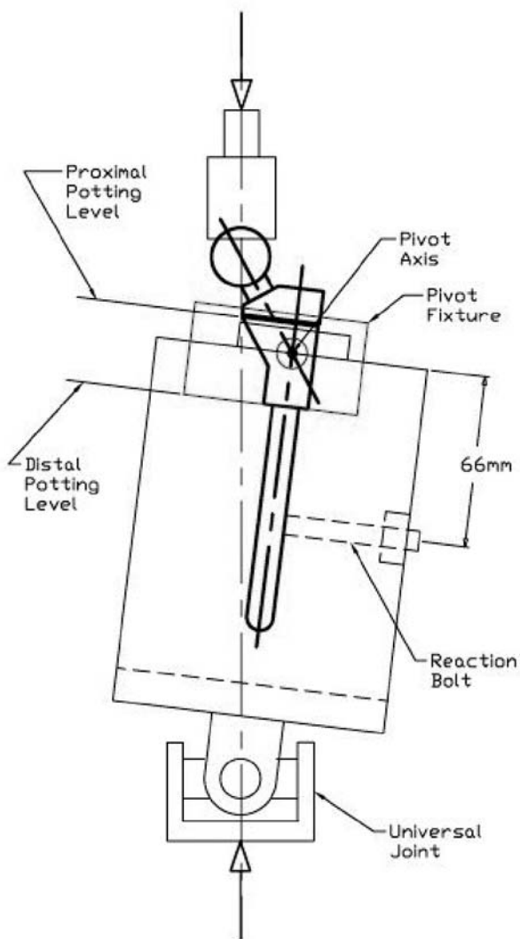
FIG. 2 Schematic Representation of the Test Set-up
