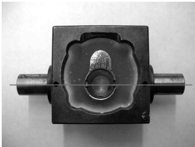
FIG. 3 Proximal Sleeve Component Potted in Pivot Fixture
