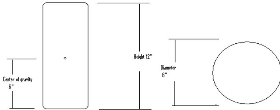
FIG. 5 Dimensions of Test Cylinder
