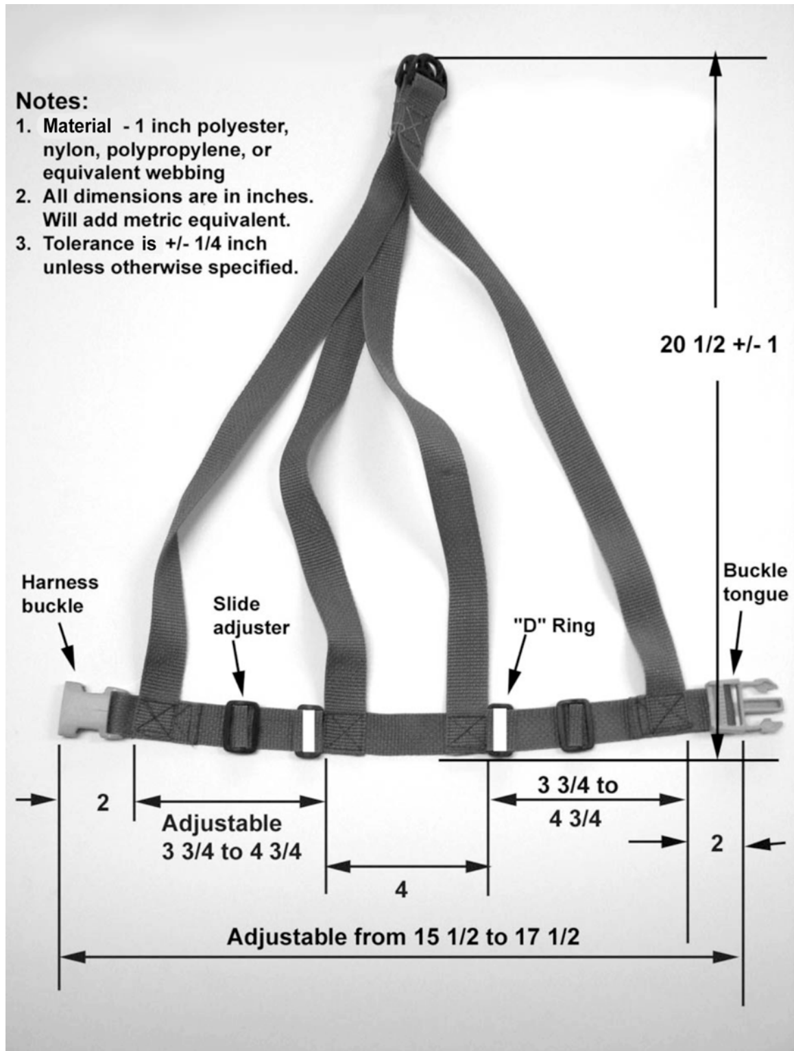
FIG. 4 Restraint System Test Harness
