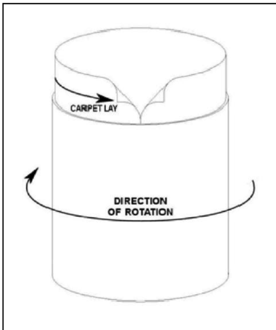
FIG. 3 Orientation of Carpet Panel in the Soiling Cylinder
