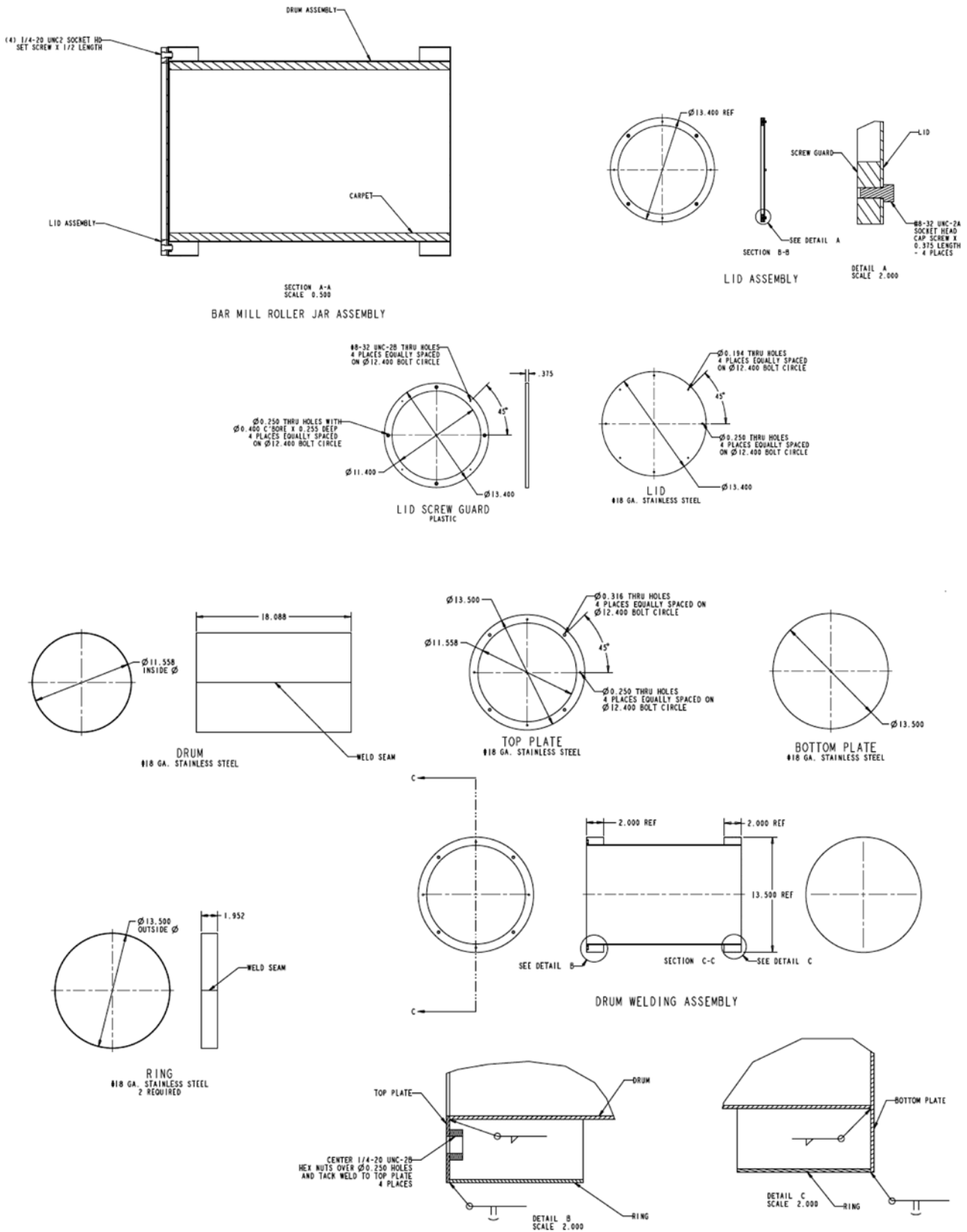
FIG. X1.1 Carpet and Pellet Soiling Cylinder
