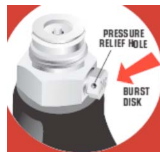
FIG. 8 Pin Valve Showing Burst Disk Assembly
