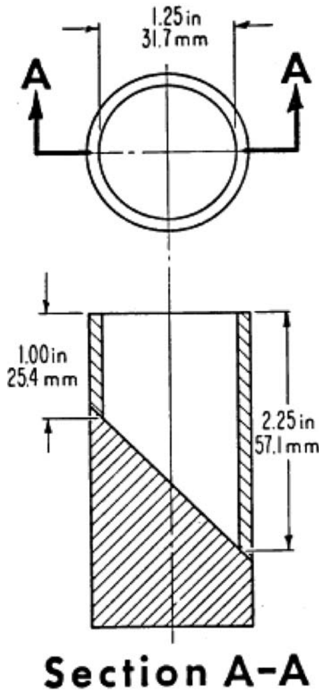
FIG. 1 Small Parts Cylinder
