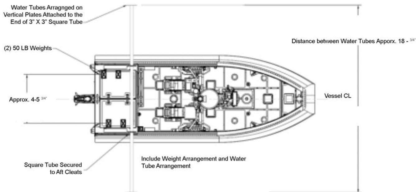
FIG. 7 Typical Water Tube Arrangements
