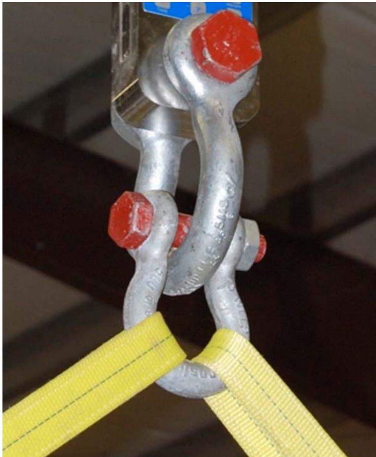
FIG. 5 Improvised "Knife-Edge" Configuration (forward and aft) Pick Points
