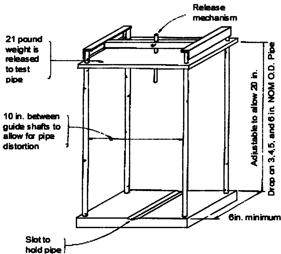
FIG. 2 Brittleness Test Device
