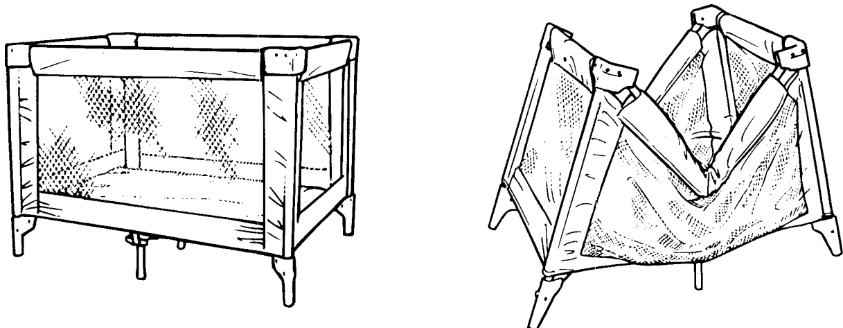
FIG. A1.3 Top Rail Assembly With Central Hinge(s) That Move Vertically Downward
