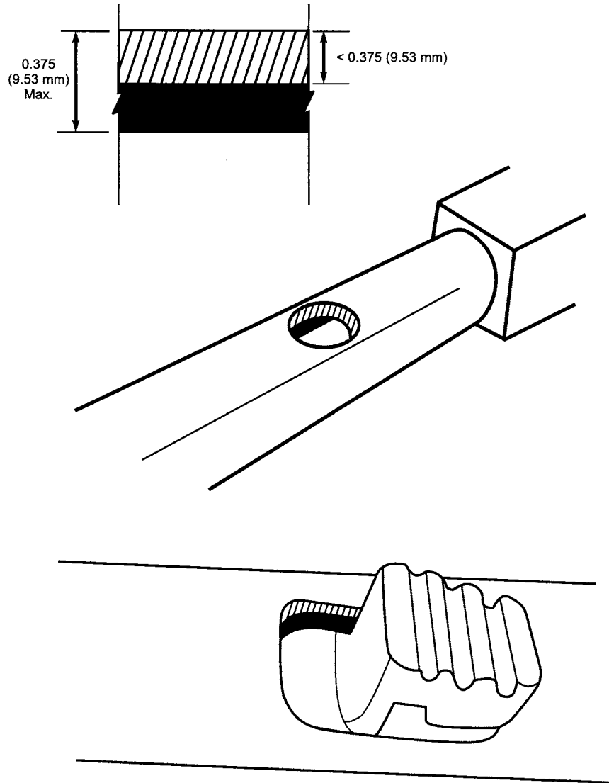
FIG. A1.4 Opening Example
