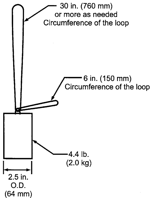
FIG. A1.31 Weight Gage
