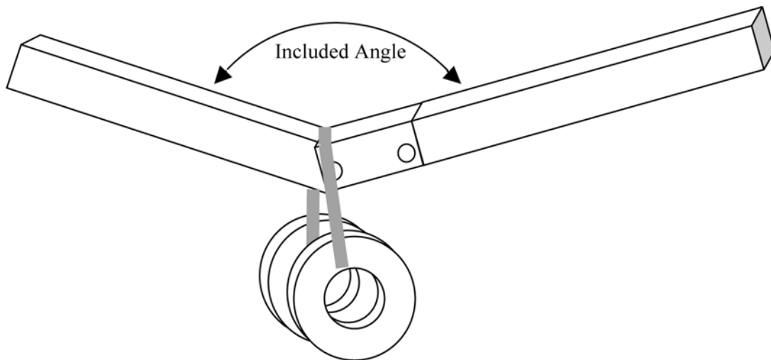
FIG. A1.35 Double Latching Device with One Latch Unlocked and 10 lbm Suspended from Hinge
