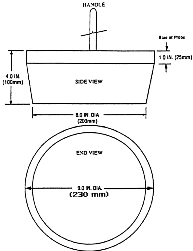
FIG. A1.8 Large Head Probe
