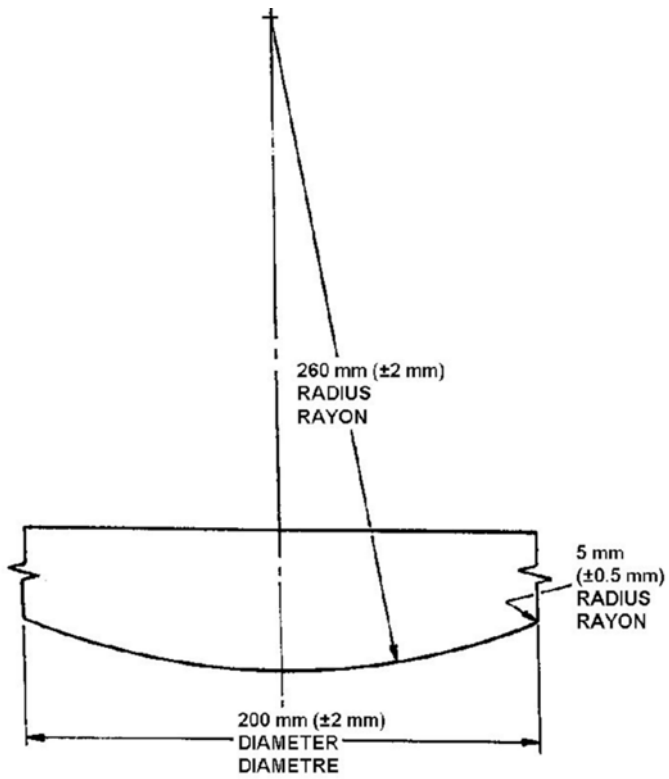
FIG. A1.20 Profile of Impact Mass
