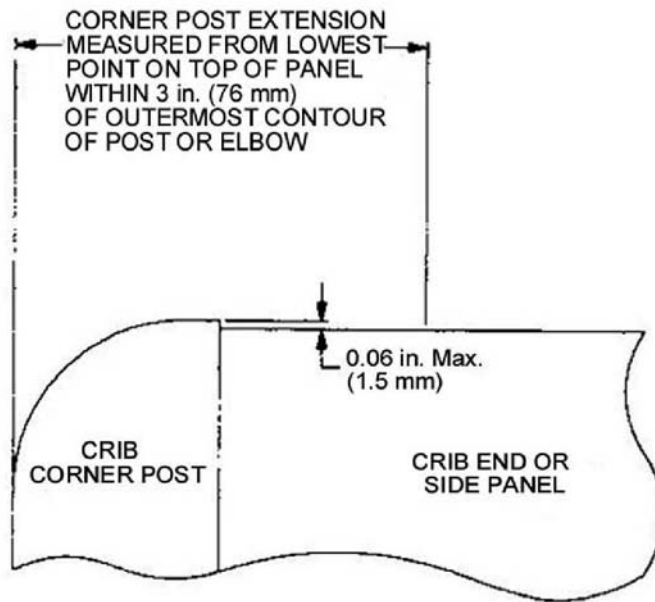
FIG. A1.2 Illustration of Requirements for Crib Corner Post Extensions
