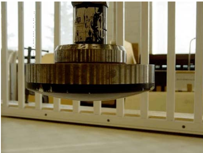
FIG. A1.21 View of Impact Mass
