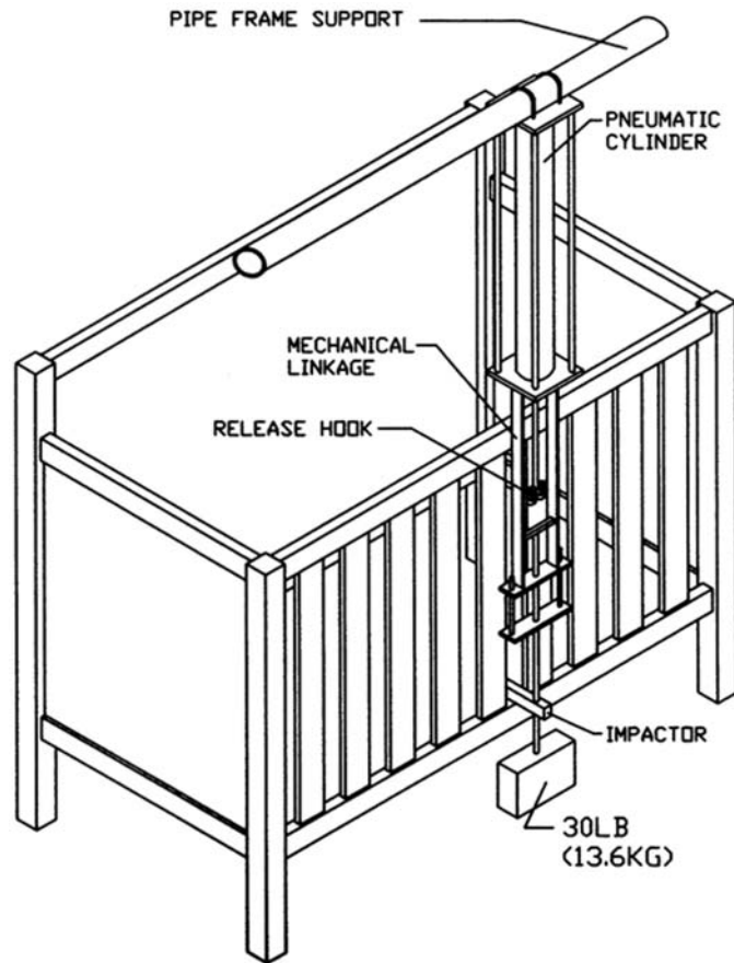
FIG. A1.25 Typical Side Assembly Test Fixture
