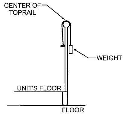
FIG. A1.32 Test over Top Rail
