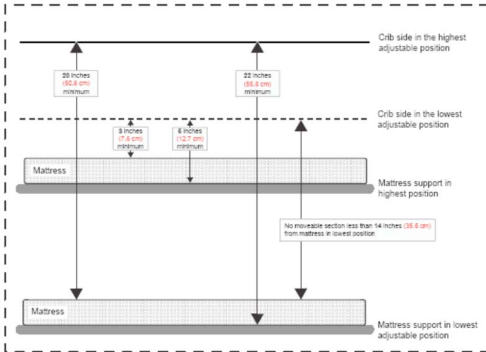
FIG. A1.11 Moveable Sides for Rigid Sided Products
