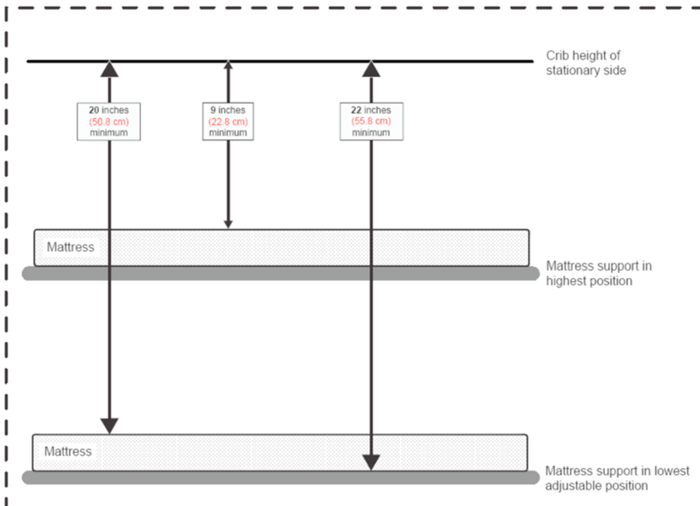
FIG. A1.12 Stationary Sides for Rigid Sided Products
