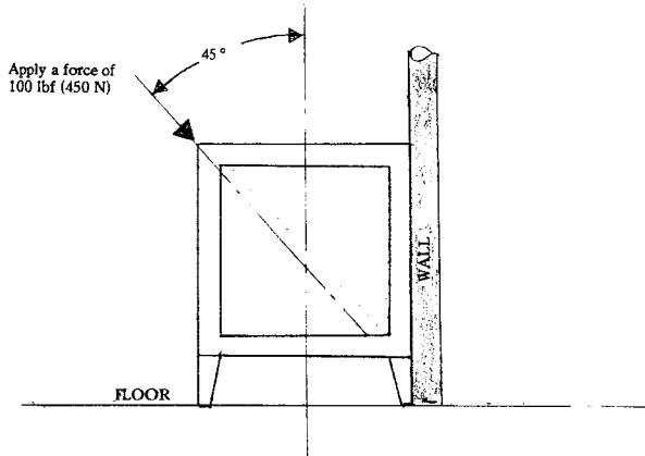
FIG. A1.26 Two Methods for Testing in Accordance with 8.11.2.4
