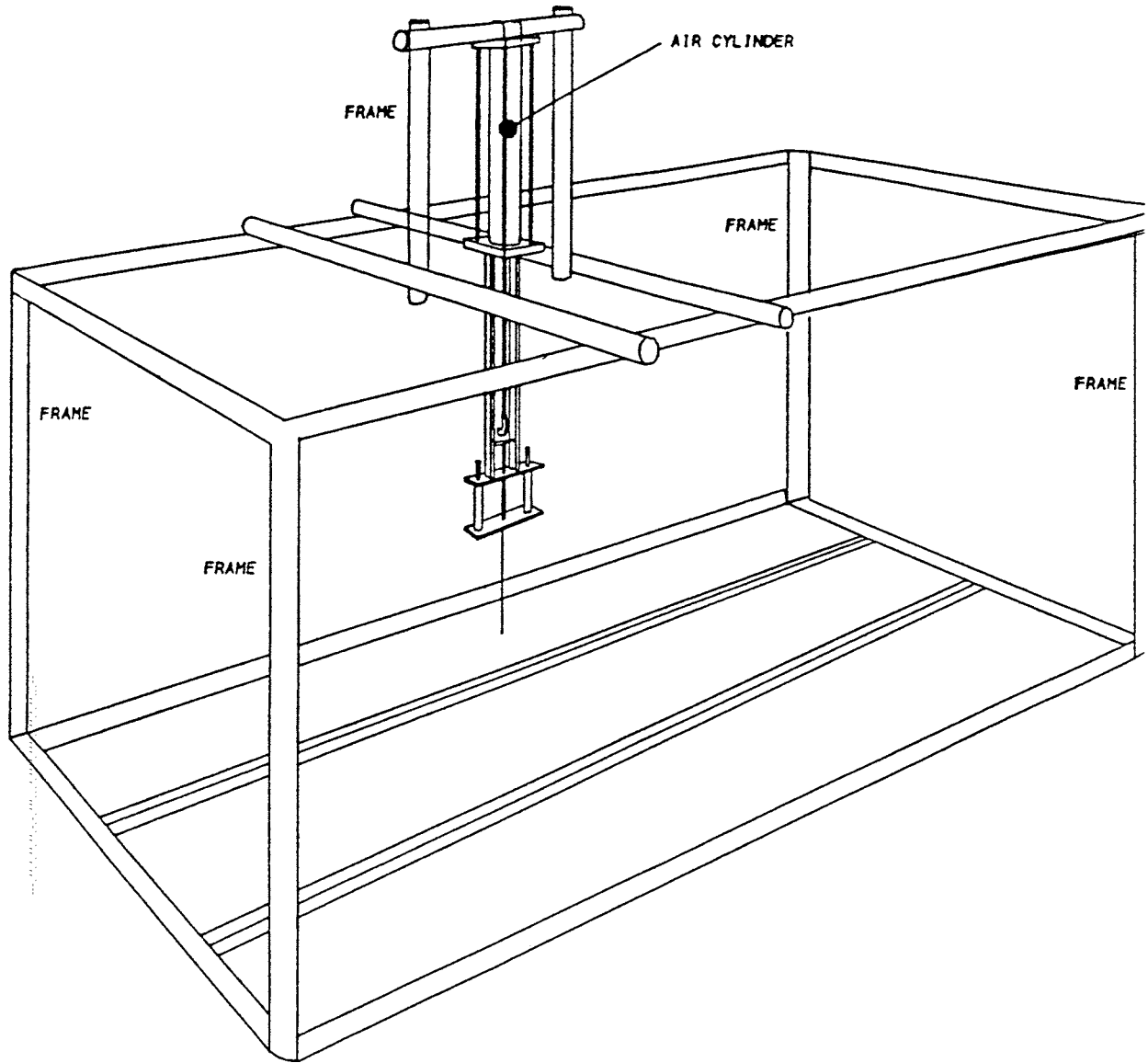
FIG. A1.19 Typical Test Frame
