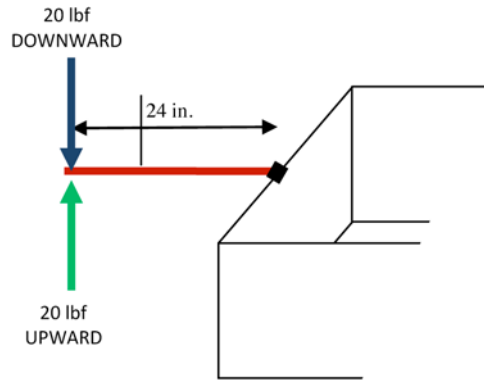
FIG. A1.37 Moment Arm Formed by Applying a 20 lbf 24 in. From the Centerline of the Top Rail
