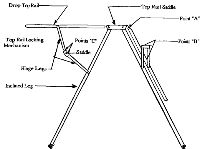
FIG. A1.3 Product Frame Components
