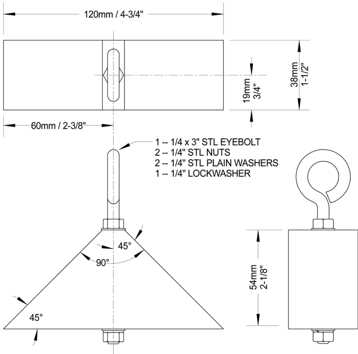
FIG. A1.13 Loading Wedge
