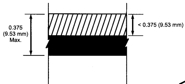
FIG. A1.4 Top Rail Assembly With Central Hinge(s) That Move Vertically Downward
