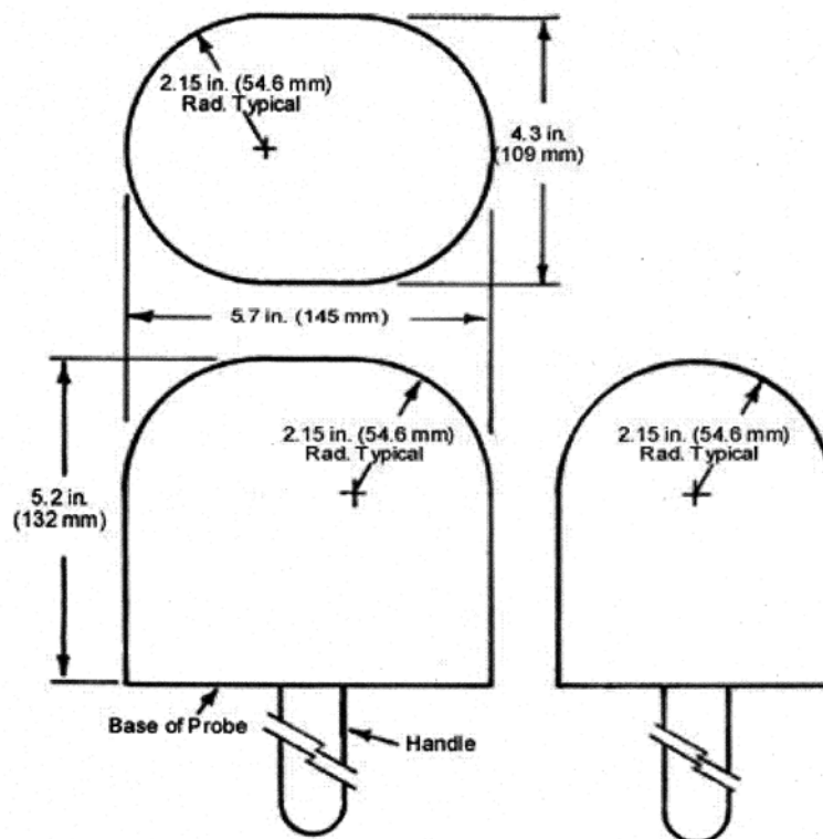
FIG. A1.7 Small Head Probe
