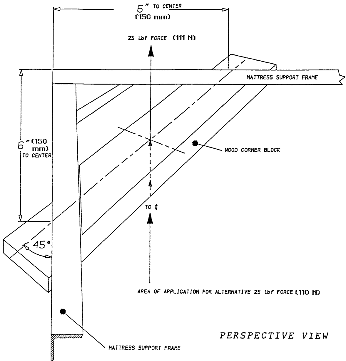
FIG. A1.24 Typical Mattress Support Detail
