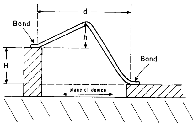
FIG. 2 Diagram of a Typical Wire Bond
