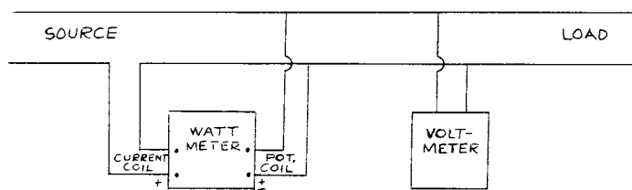
FIG. 1 Schematic Diagram of Meter Connections
