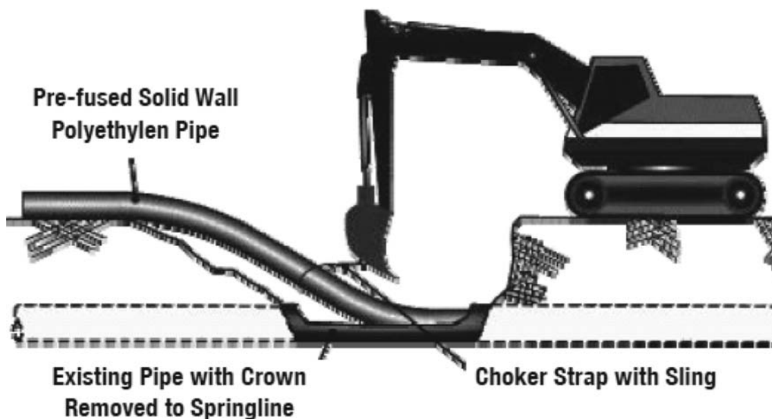
FIG. 7 Alternate Push Technique
