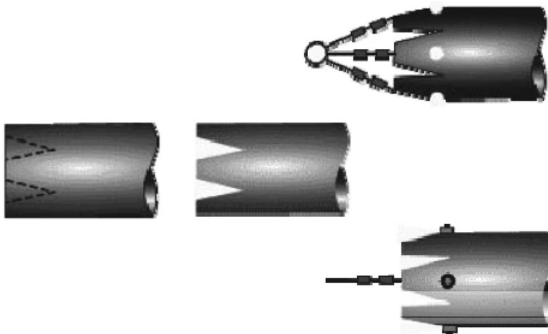
FIG. 6 Field Fabricated Pulling Head
