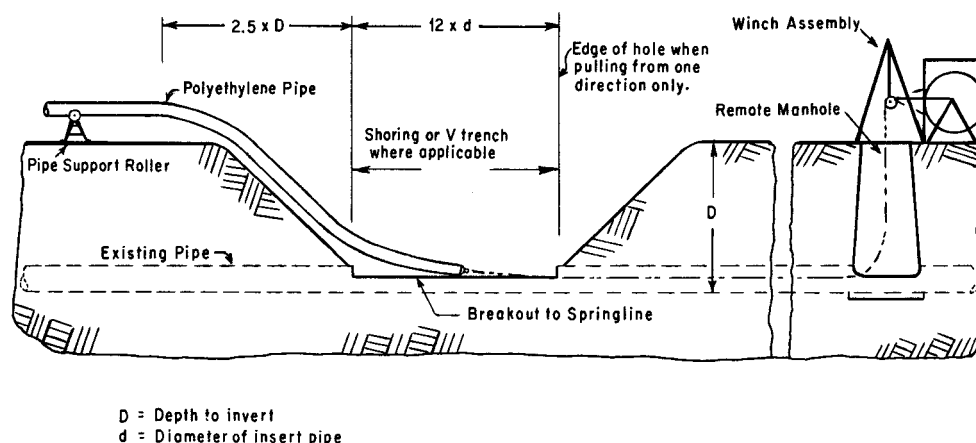
FIG. 1 Insertion Hole and Pull-in Detail
