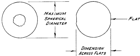
FIG. 2 Air-Gun Shot
