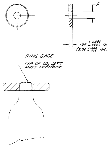
FIG. 4 CO 2 (Carbon Dioxide) Cylinder Non-Refillable
