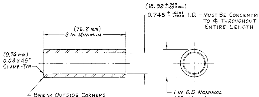
FIG. 7 Ring Gage—CO 2 Cylinder Non-Refillable Diameter
