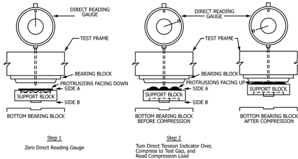
FIG. 20 Steps for Determining Compression Load
