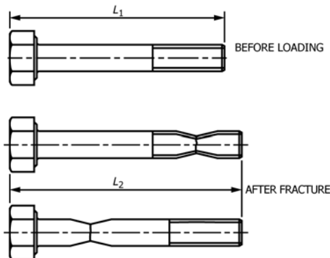
FIG. 11 Determination of Total Extension at Fracture ( A_L ) (only Screw Product Shown)
