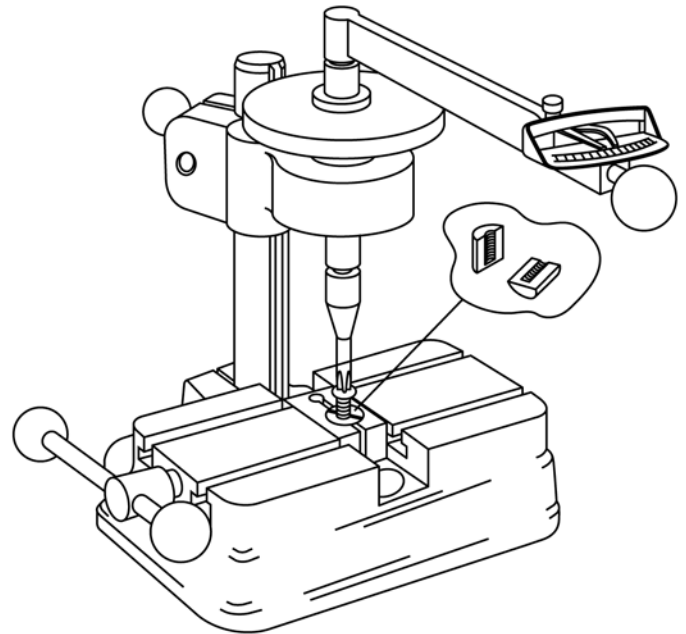
FIG. 22 Typical Torsional Strength Test Fixture
