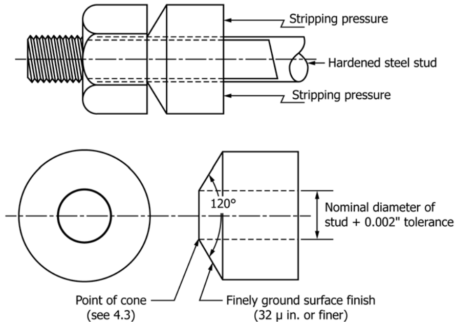
FIG. 16 Cone-Proof Test
