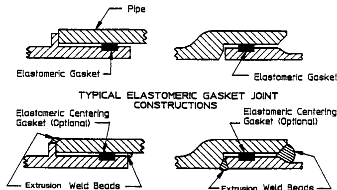
FIG. 2 Typical Extrusion Weld Joint Constructions
