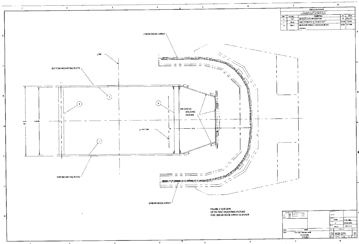
FIG. 3 Side View of Pie Disk Mounting Fixture for Linear Diode Array Scanner
