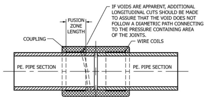
FIG. 16 Coupling Fusion Assembly—Further Examination Guidance
