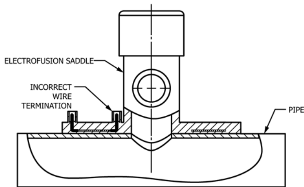
FIG. 5 Incorrect Wire Termination Saddle—Single Coil
