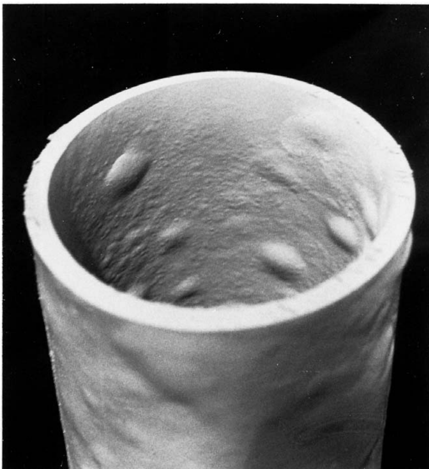
FIG. X1.5 Internal Blistering
