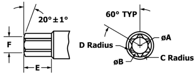
FIG. 6 Dimensions of Hexalobe Screwdriver Bits
